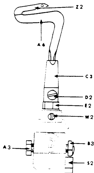
Fig. 32. Left Looper Assembly
