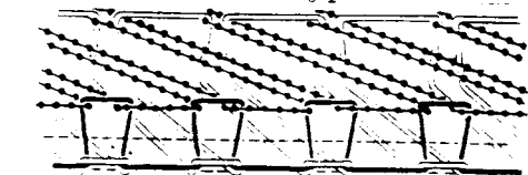
Fig.6. Stitch Formation (Stitch Type No.505)
