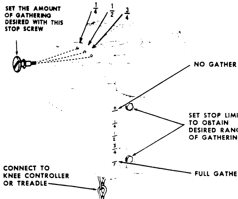
Fig. 46. Intermittent Gathering Feed Mechanism.
