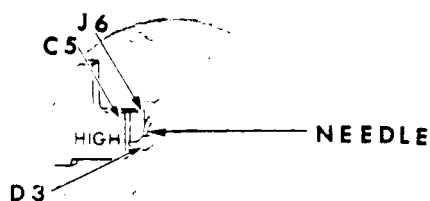
Fig. 36. Right Looper (Left Position) and Gauge 82253 or 82254 (Two Needle)
