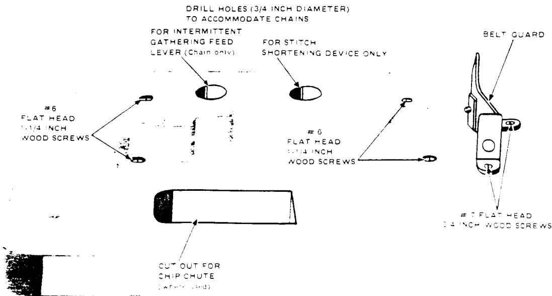
Fig. 9. Machine Cutout, Showing Position and Drill Sizes of Holes Required for Installation.
