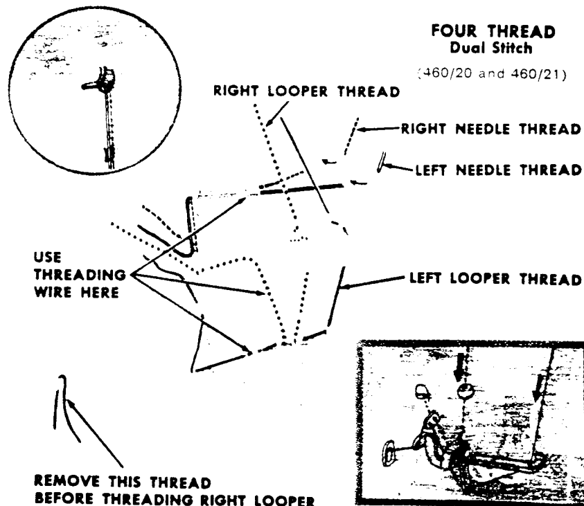
Fig. 21. Threading the Machine. (Four-Thread Dual Stitch)
