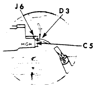
Fig. 35. Right Looper (Left Position) and Gauge 82253 or 82254 (Single Needle).
