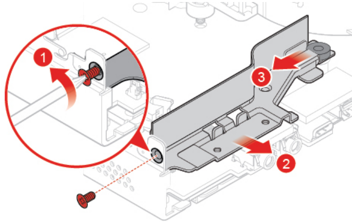
Figure 82. Removing the antenna bracket
